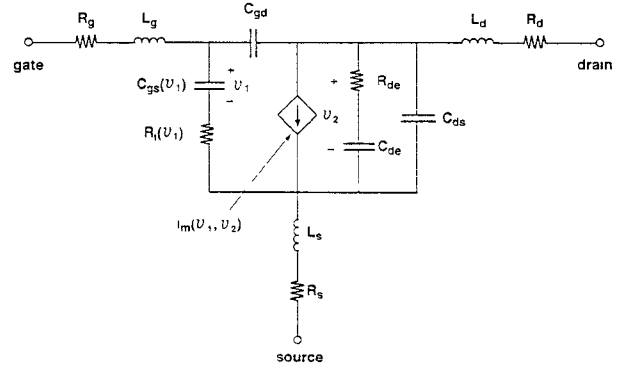
Fig. 1 A large-signal MESFET model used for the mixer example. All parameter values are consistent with [8].
